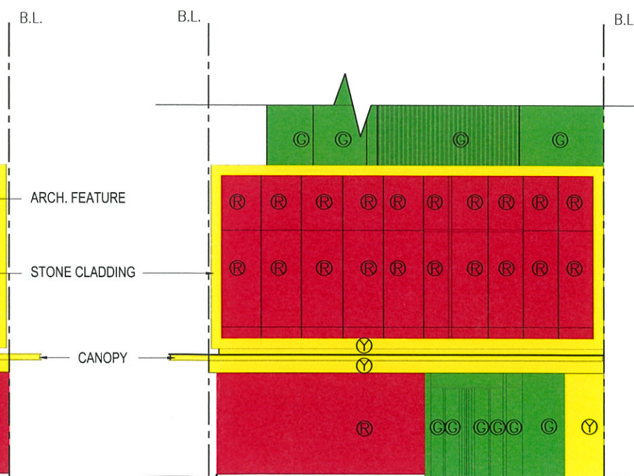
NORTH - EAST ELEVATION (FACING TAI SHEK STREET)
