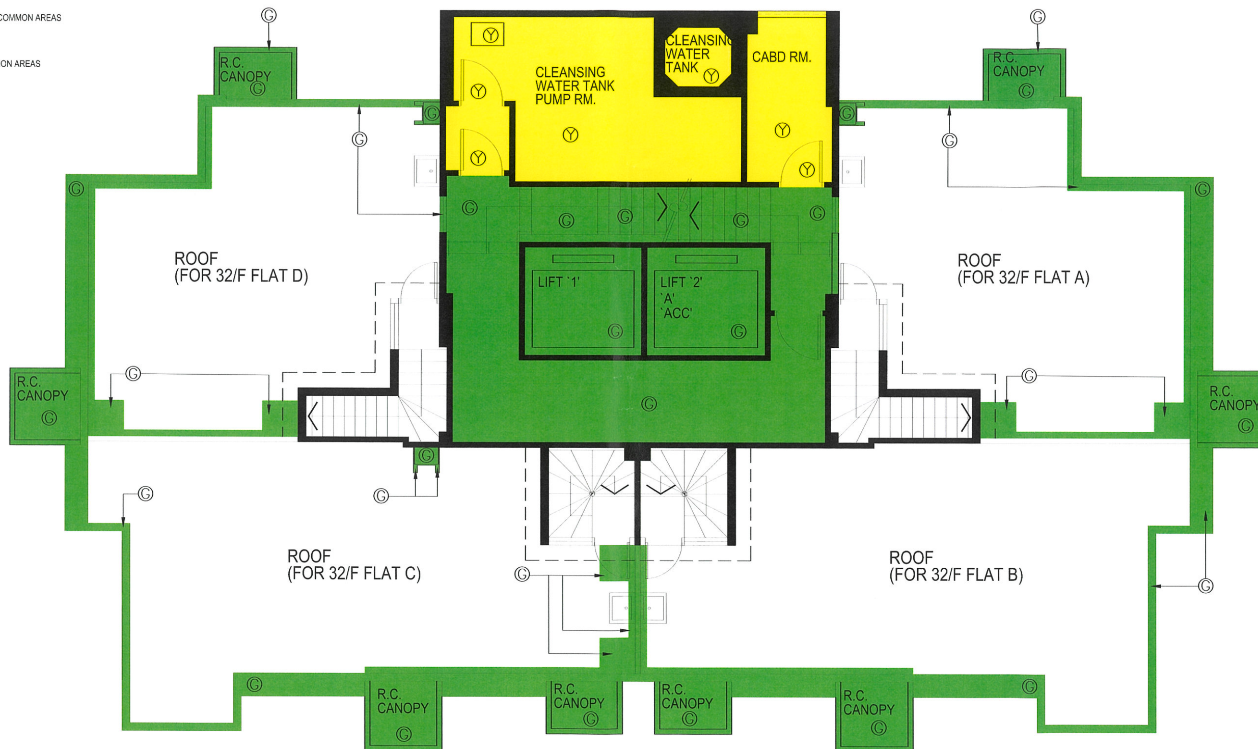
ROOF PLAN ( PLAN NO. DMC-10)
