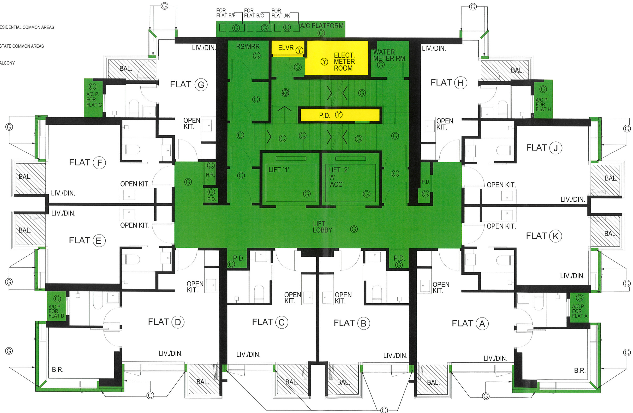
7TH - 13TH, 15TH - 16TH, 18TH - 23RD, 25TH - 31ST FLOOR PLAN ( PLAN NO. DMC-07)
