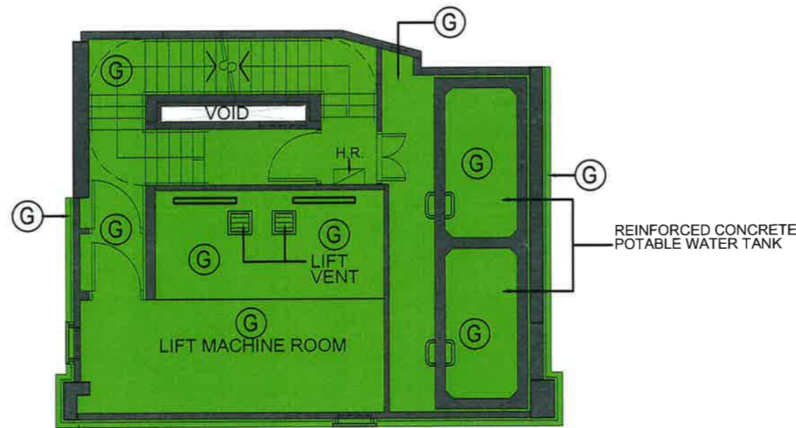
PLAN OF LEVEL 111.580
