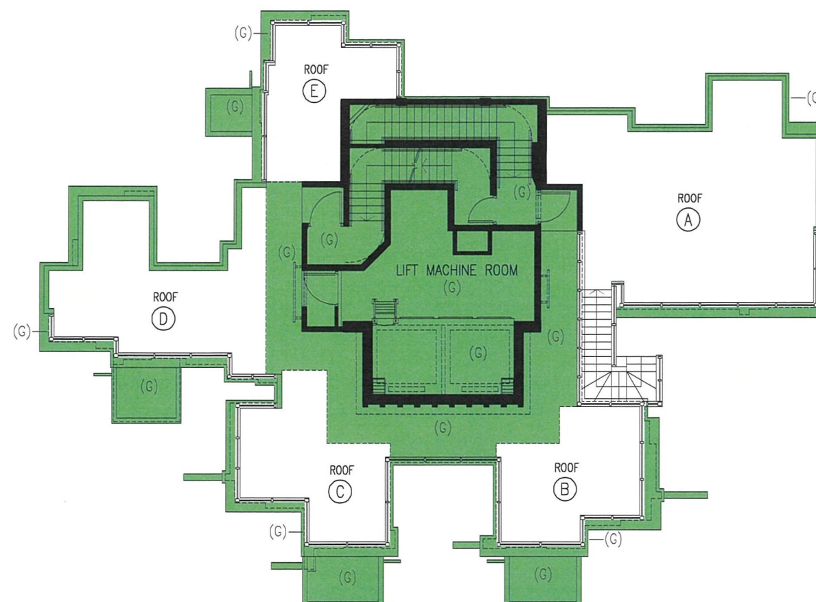
TOWER 1 – ROOF DMC PLAN FOR IDENTIFICATION PURPOSE ONLY
