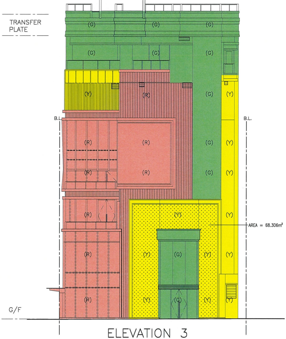
ELEVATION 3 (FACING KWEILIN STREET) FOR IDENTIFICATION PURPOSE ONLY
