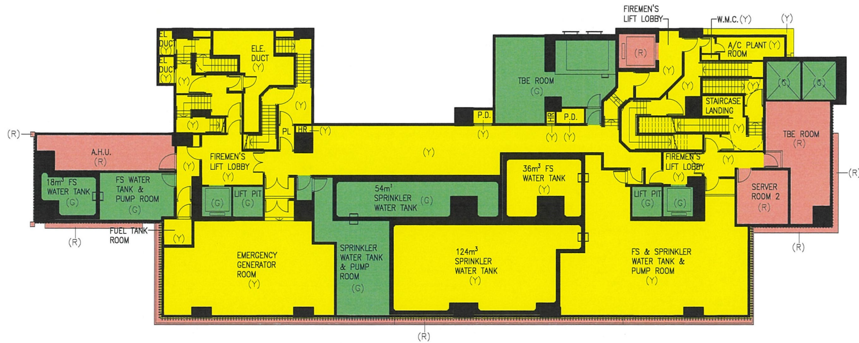
5/F DMC PLAN FOR IDENTIFICATION PURPOSE ONLY
