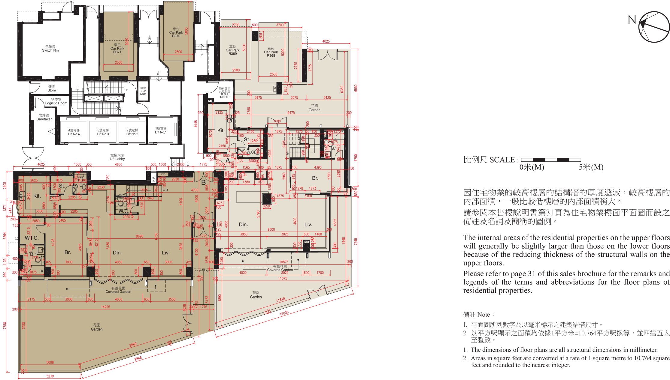
地下之現狀間隔平面圖 (複式低層) AS-IS FLOOR PLAN FOR GROUND FLOOR (LOWER DUPLEX)
