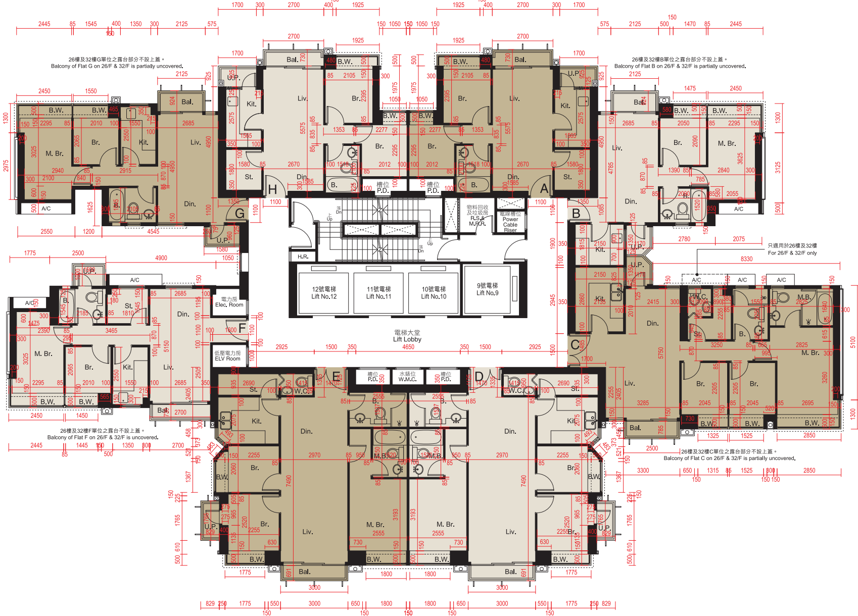
25樓 - 26樓及29樓 - 32樓平面圖 25TH - 26TH & 29TH - 32ND FLOOR PLAN
