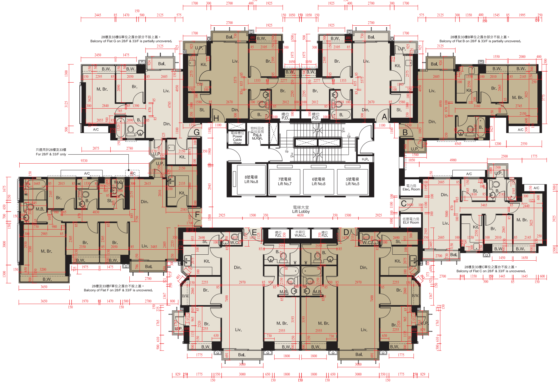
25樓 - 28樓及31樓 - 33樓平面圖 25TH - 28TH & 31ST - 33RD FLOOR PLAN
