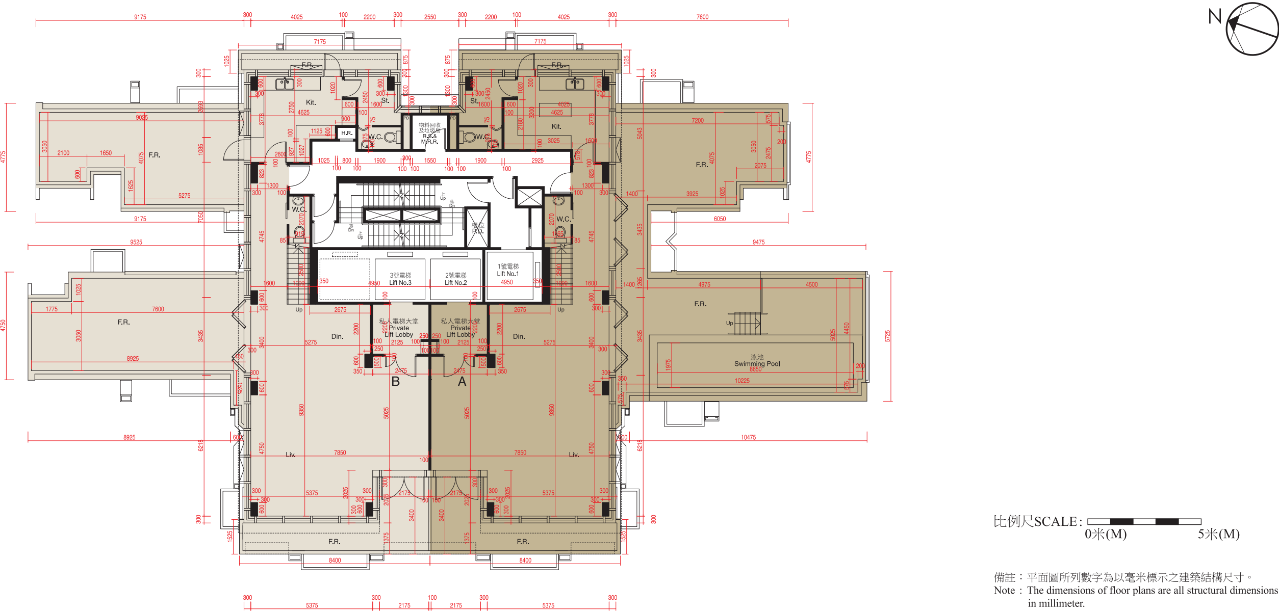
39樓平面圖 (複式低層) 39TH FLOOR PLAN (LOWER DUPLEX)
