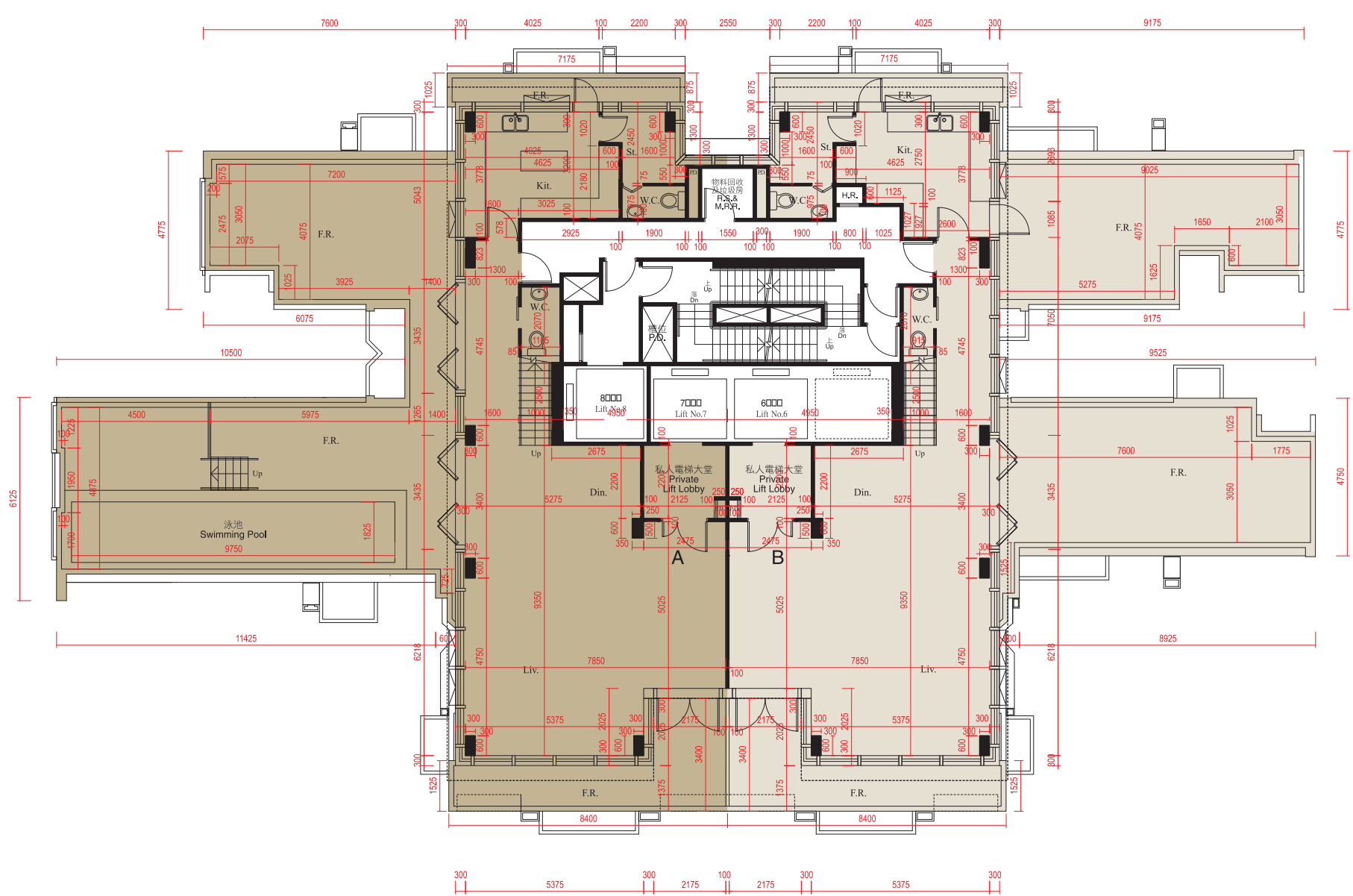
37樓平面圖 (複式低層) 37TH FLOOR PLAN (LOWER DUPLEX)
