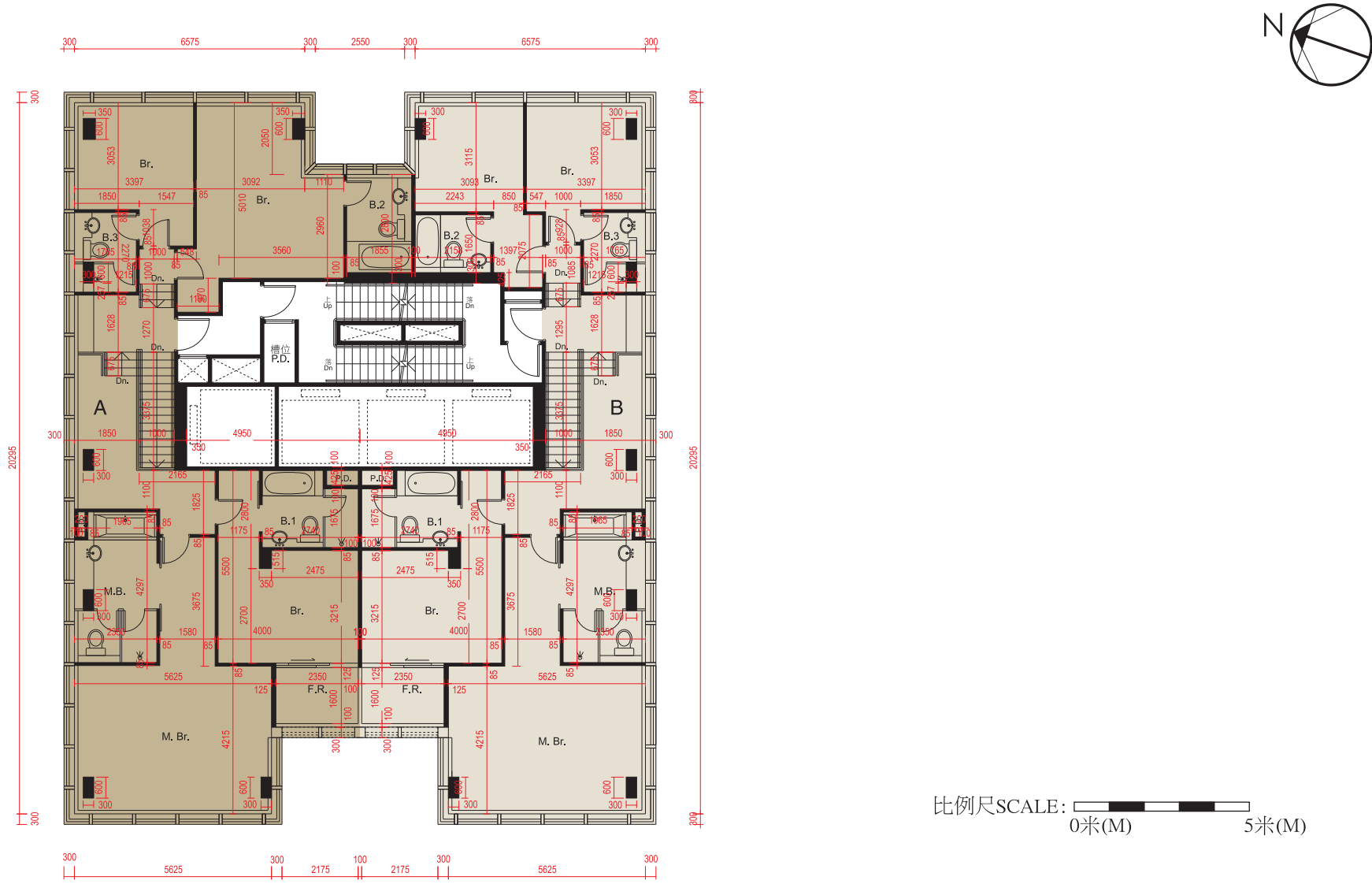
38樓平面圖 (複式高層) 38TH FLOOR PLAN (UPPER DUPLEX)
