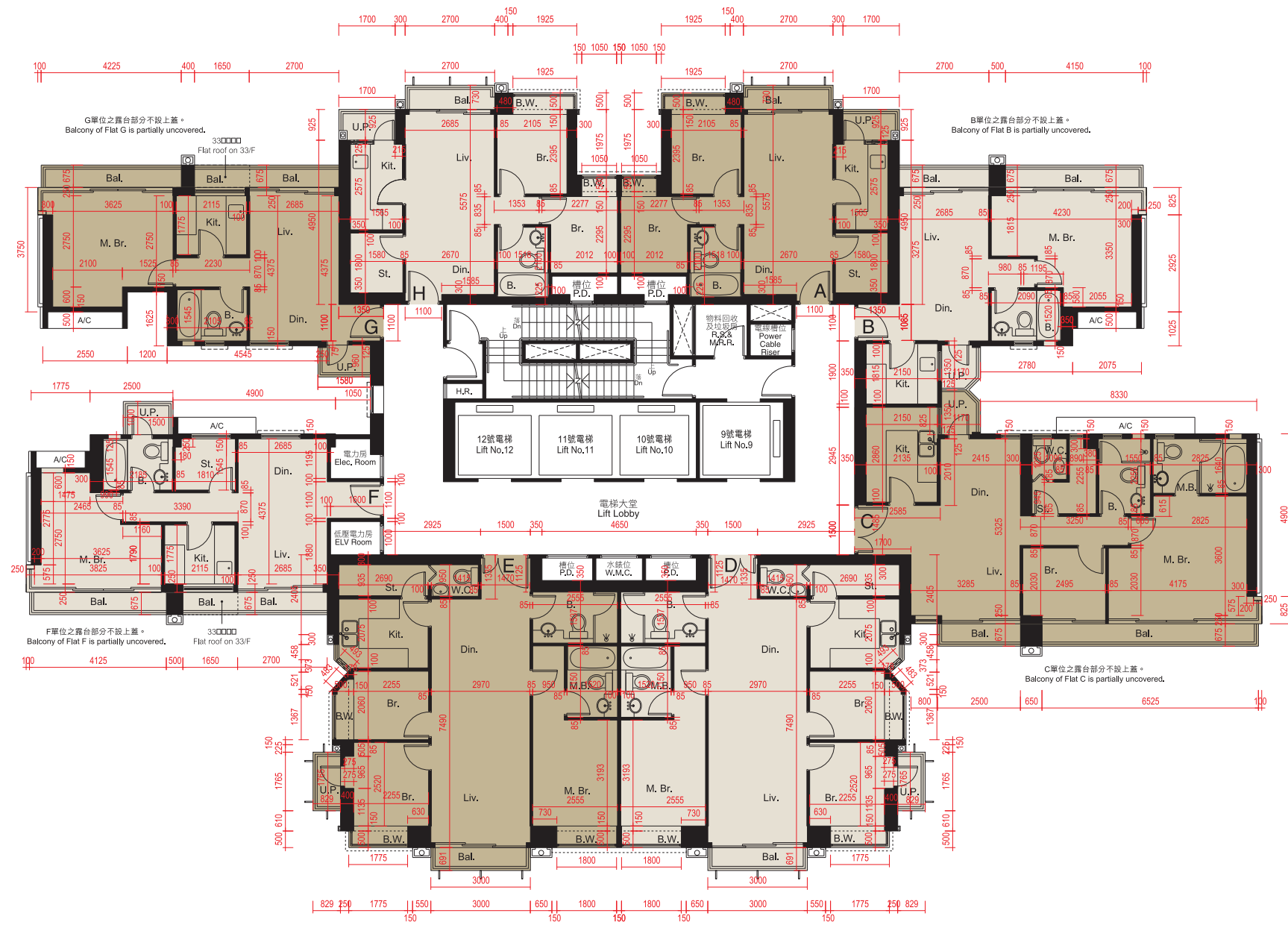
27樓及33樓平面圖 27TH & 33RD FLOOR PLAN
