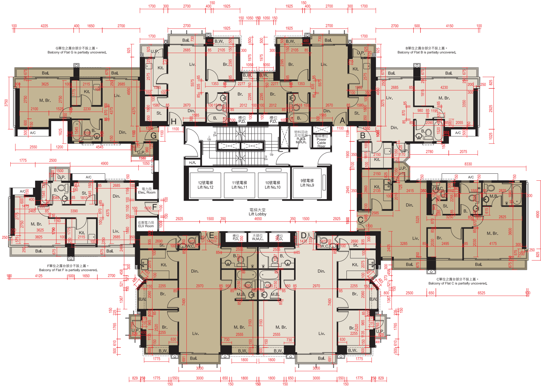
10樓及19樓平面圖 10TH & 19TH FLOOR PLAN
