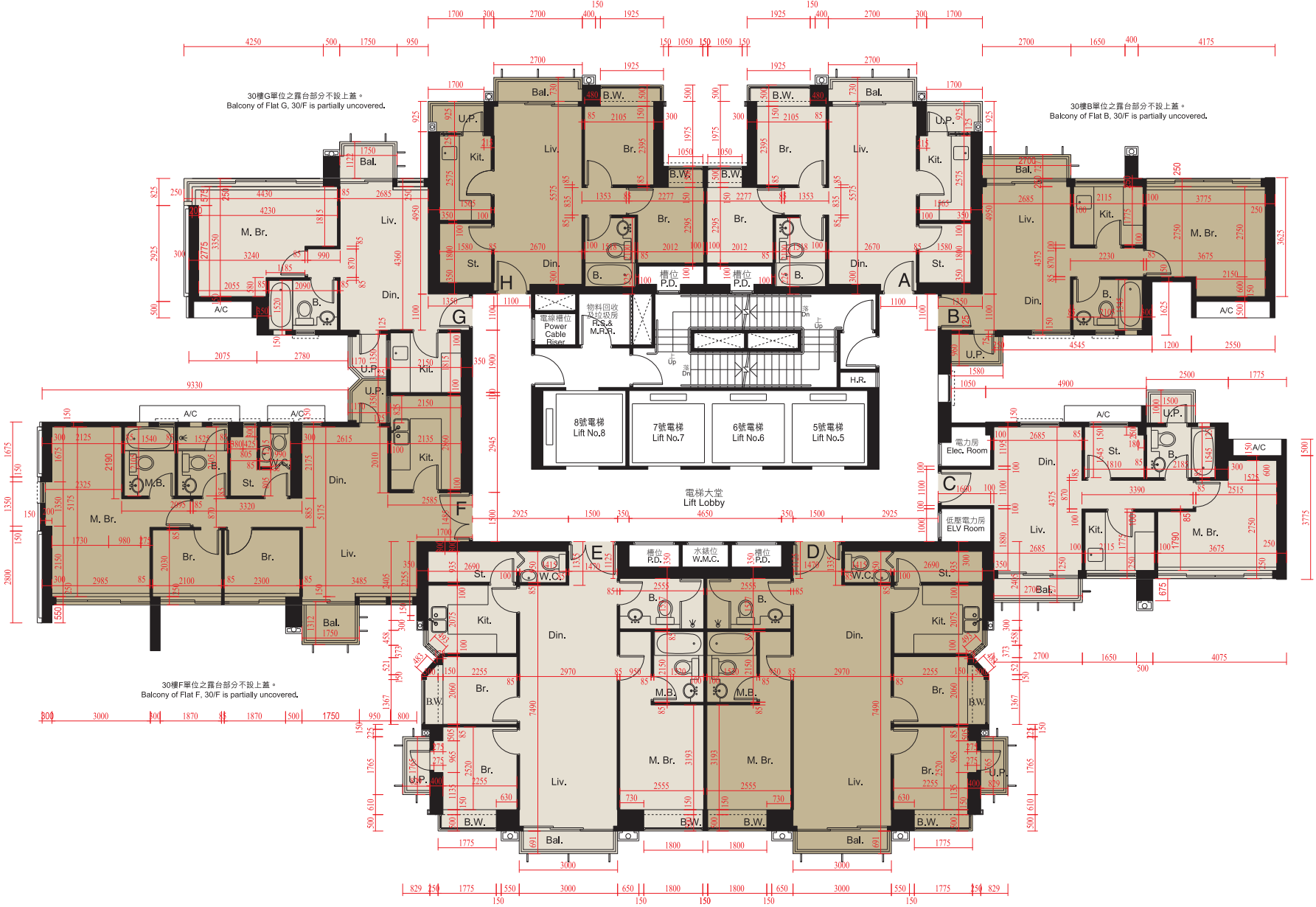
30樓及36樓平面圖 30TH & 36TH FLOOR PLAN
