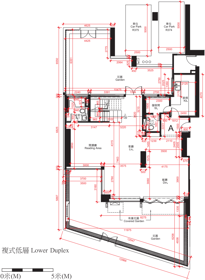
地下及1樓A單位之現狀間隔平面圖 FLAT A, G/F & 1/F AS IS FLOOR PLAN
