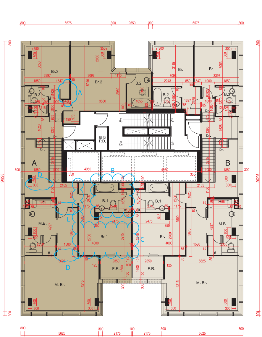
35樓平面圖 (複式高層) 35TH FLOOR PLAN (UPPER DUPLEX)
