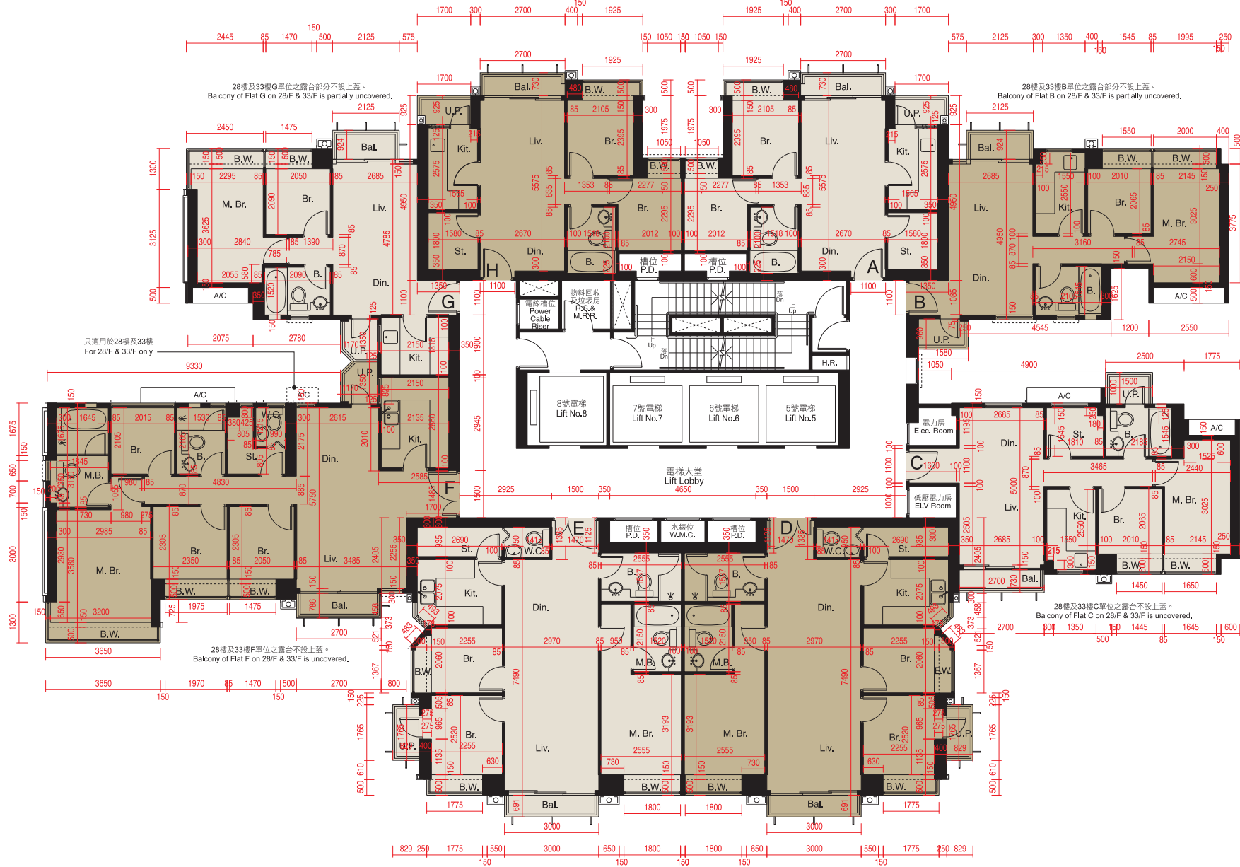
25樓 - 28樓及31樓 - 33樓平面圖 25TH - 28TH & 31ST - 33RD FLOOR PLAN
