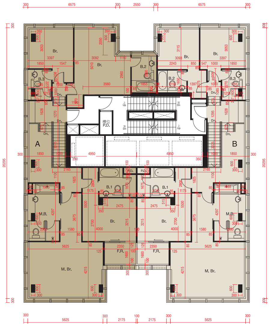
38樓平面圖 (複式高層) 38TH FLOOR PLAN (UPPER DUPLEX)
