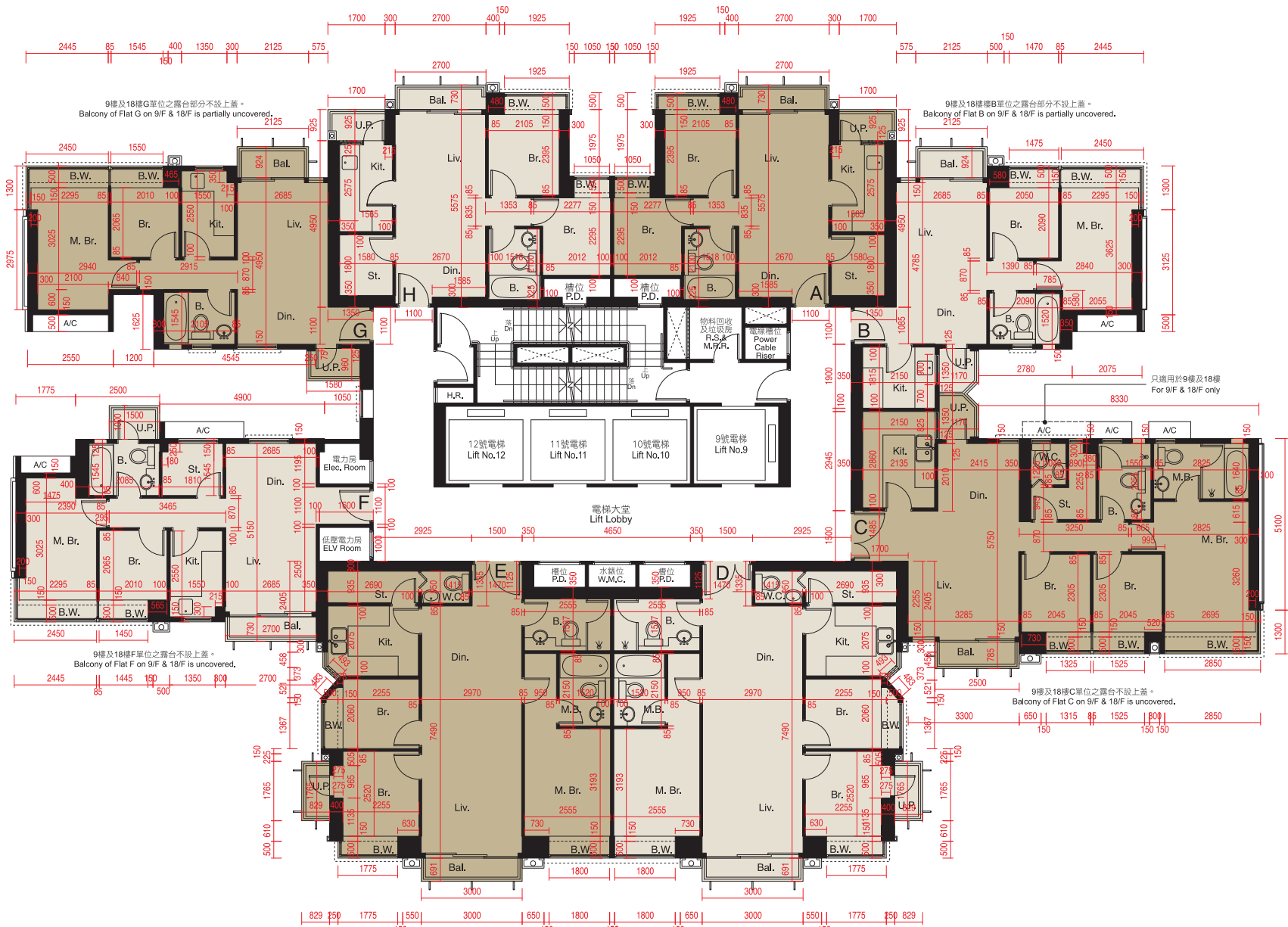
5樓 - 9樓，12樓，15樓 - 18樓及21樓 - 23樓平面圖 5TH - 9TH, 12TH, 15TH - 18TH & 21ST - 23RD FLOOR PLAN
