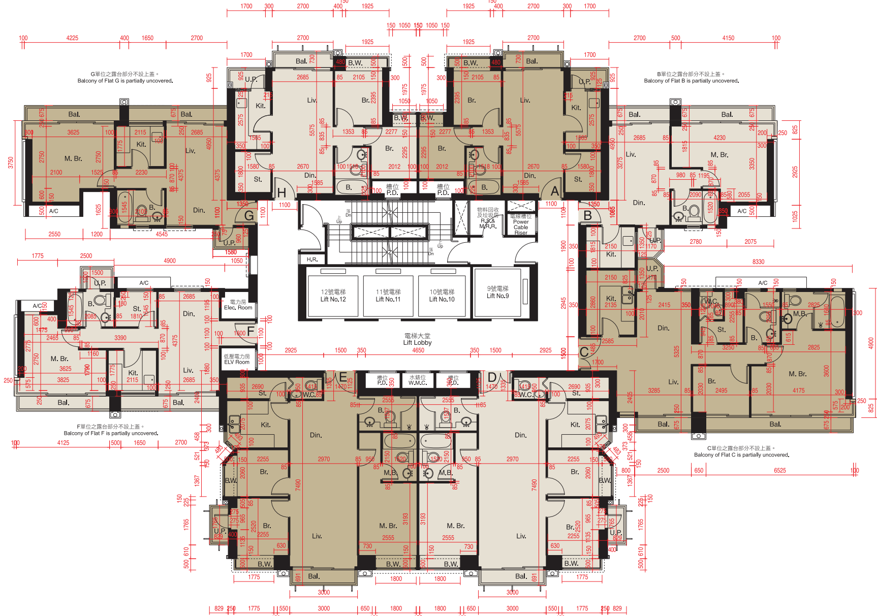
10樓及19樓平面圖 10TH & 19TH FLOOR PLAN
