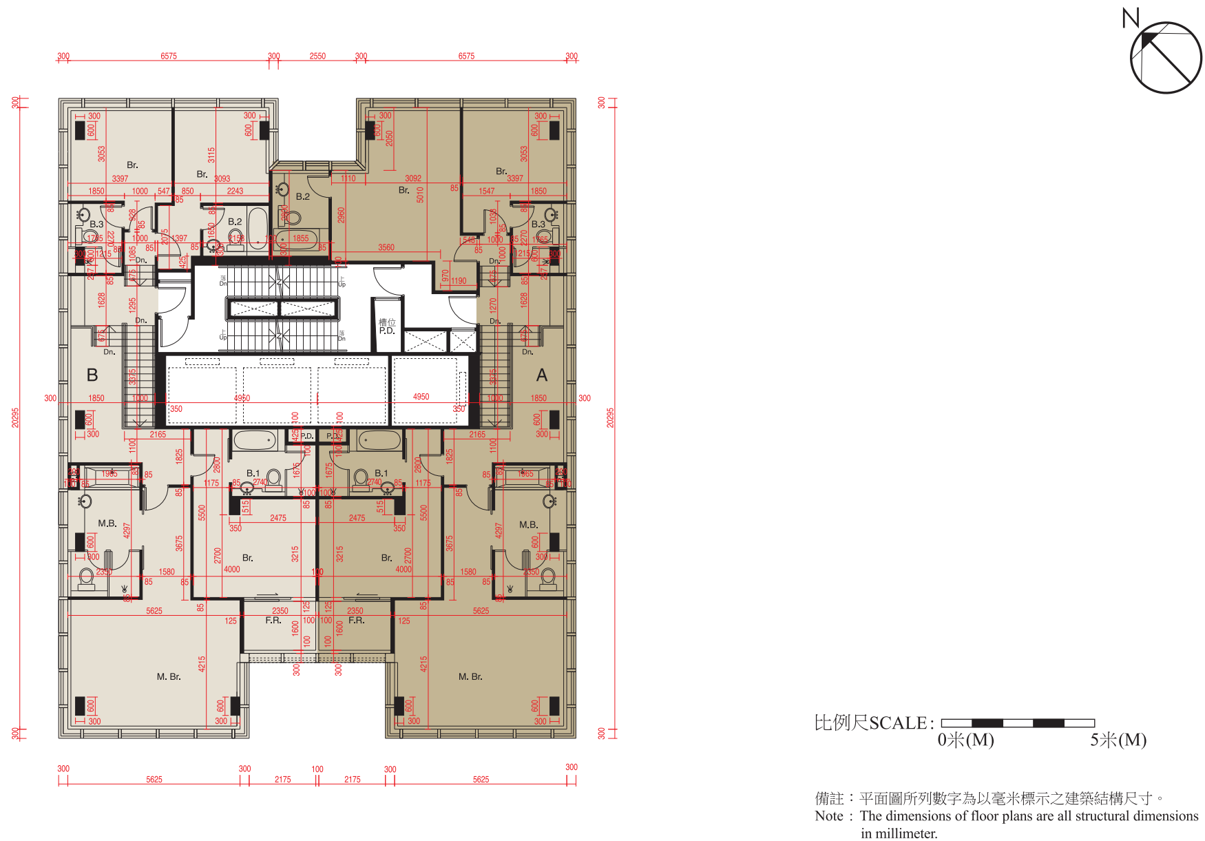
37樓平面圖 (複式高層) 37TH FLOOR PLAN (UPPER DUPLEX)
