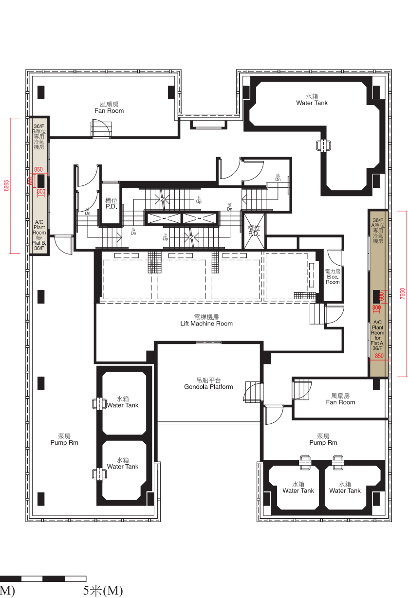
機電層平面圖 ELECTRICAL & MECHANICAL FLOOR PLAN
