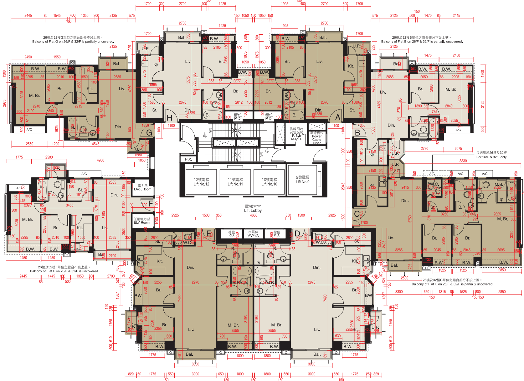
25樓 - 26樓及29樓 - 32樓平面圖 25TH - 26TH & 29TH - 32ND FLOOR PLAN
