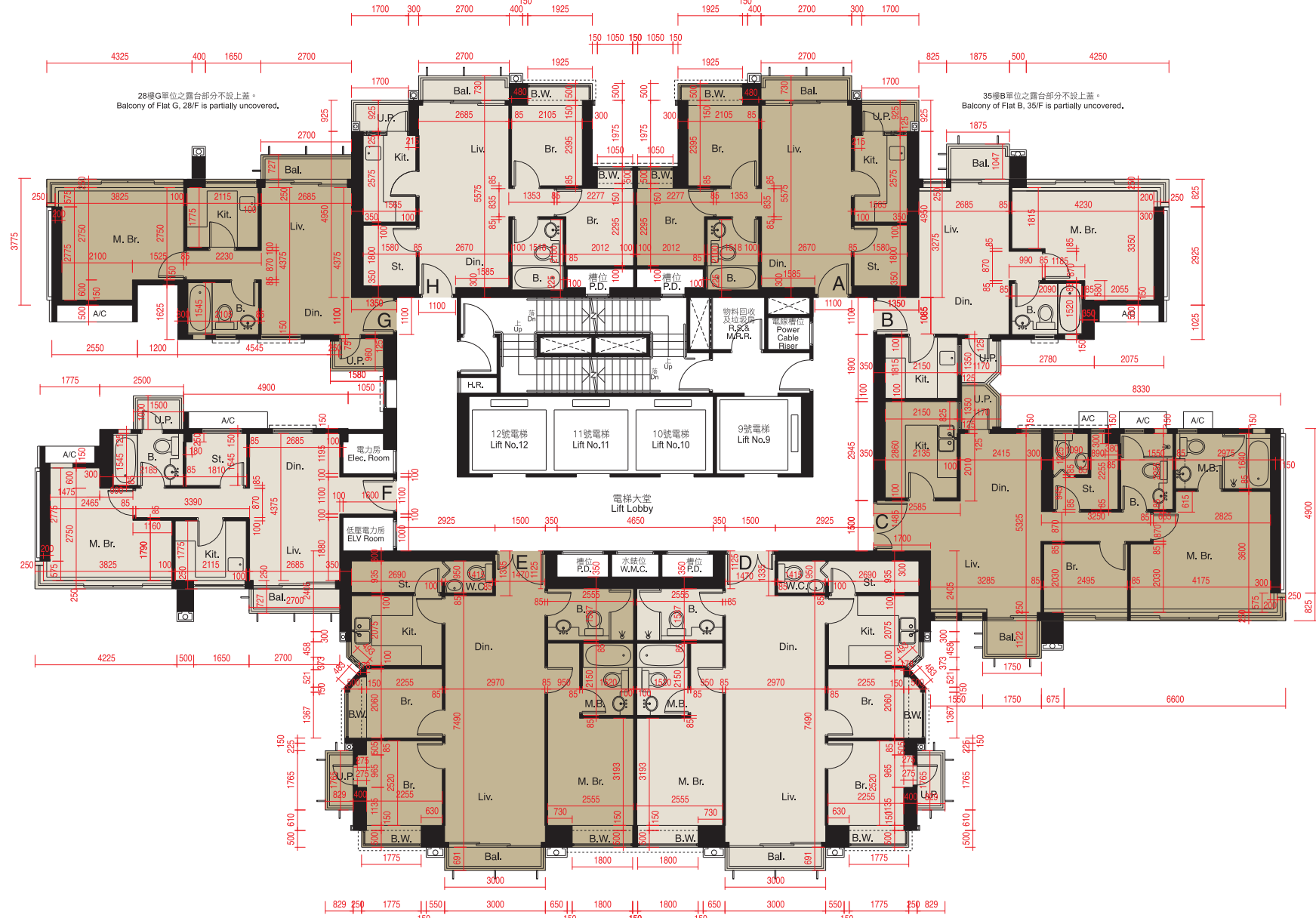
28樓及35樓平面圖 28TH & 35TH FLOOR PLAN
