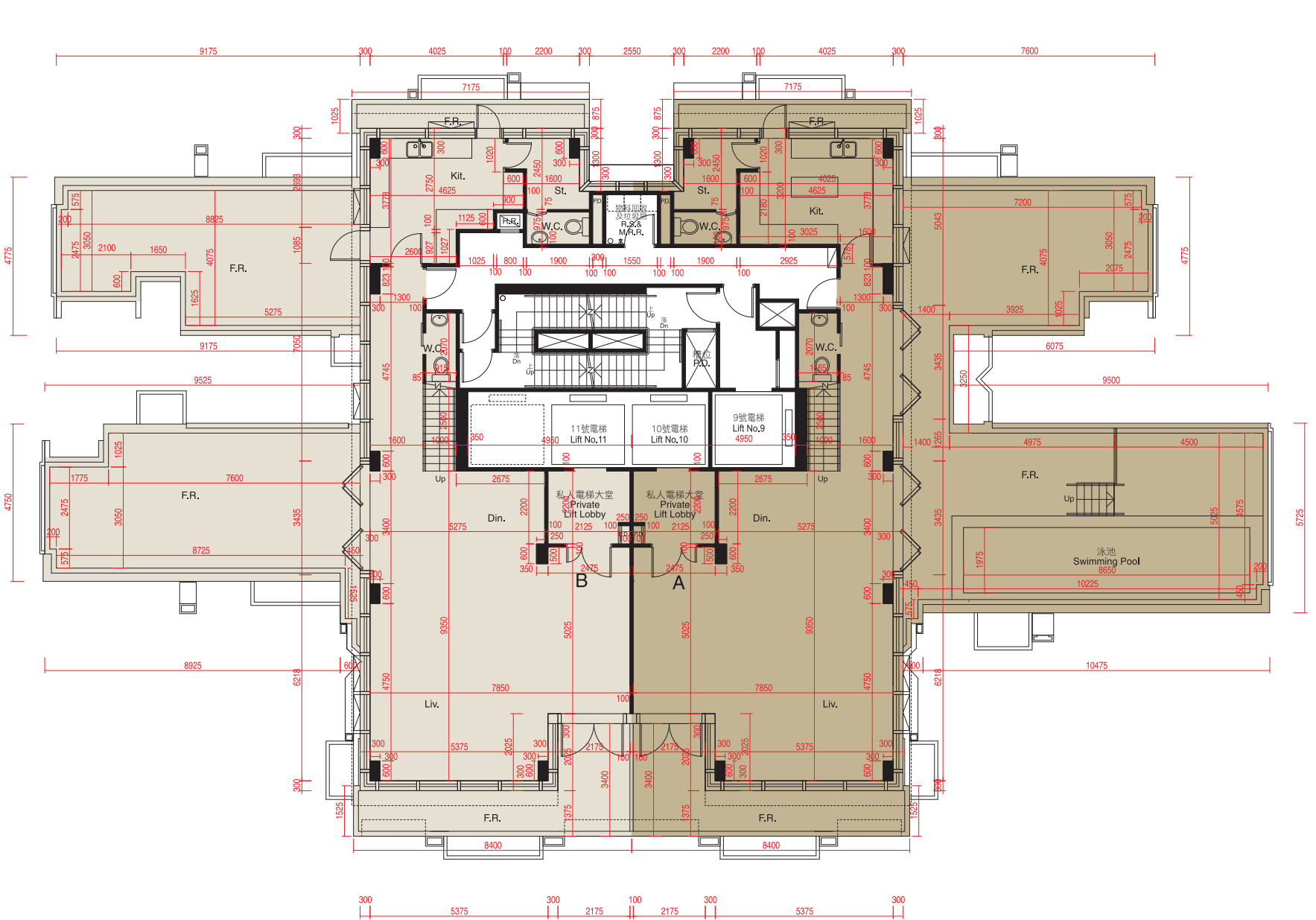
36樓平面圖 (複式低層) 36TH FLOOR PLAN (LOWER DUPLEX)
