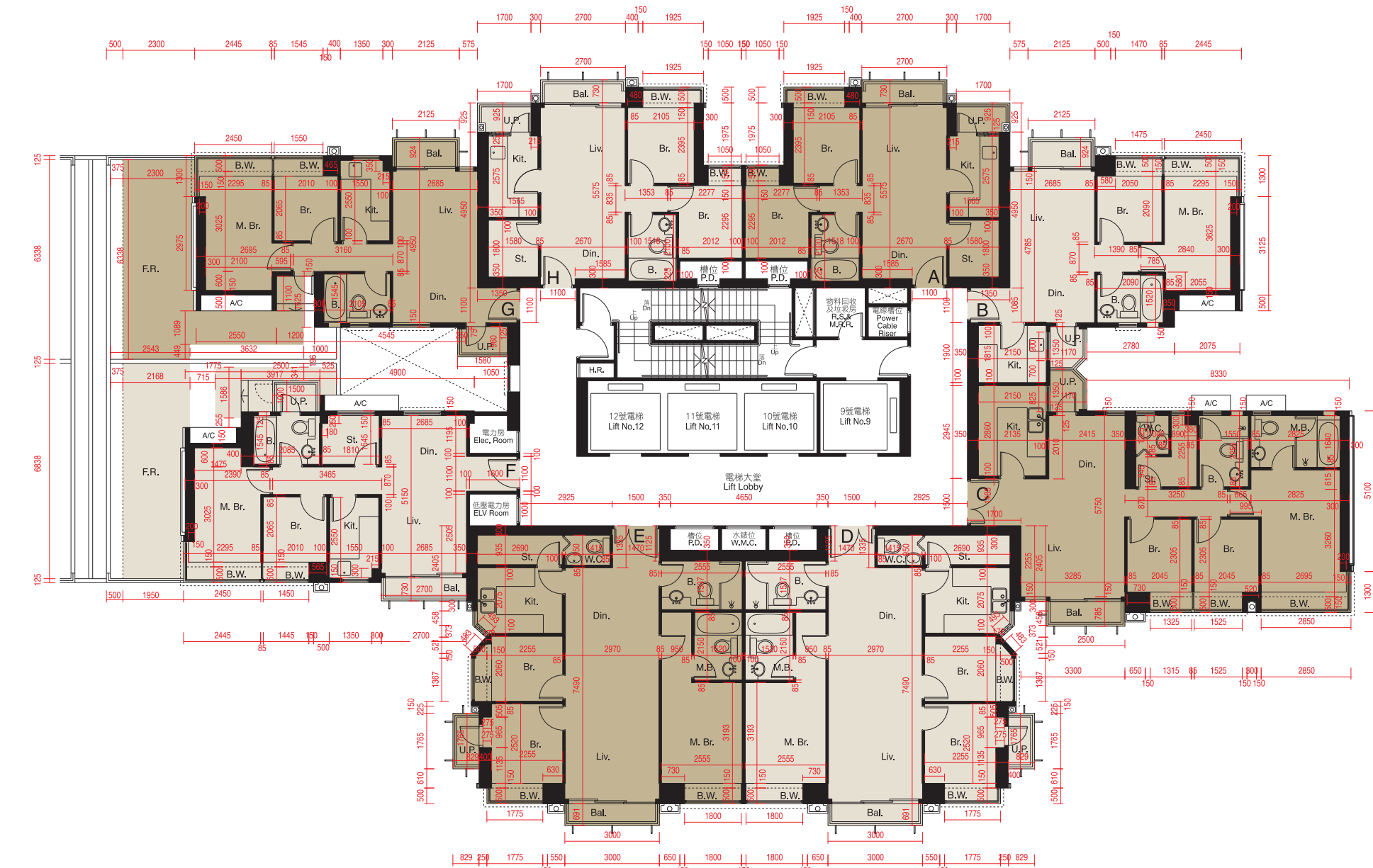
3樓平面圖 3RD FLOOR PLAN
