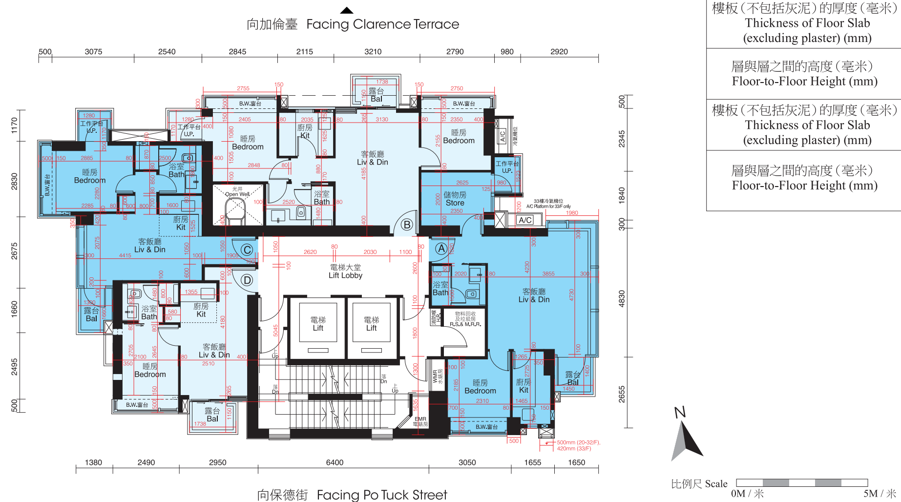
20樓至33樓平面圖 20th to 33rd Floor Plan
