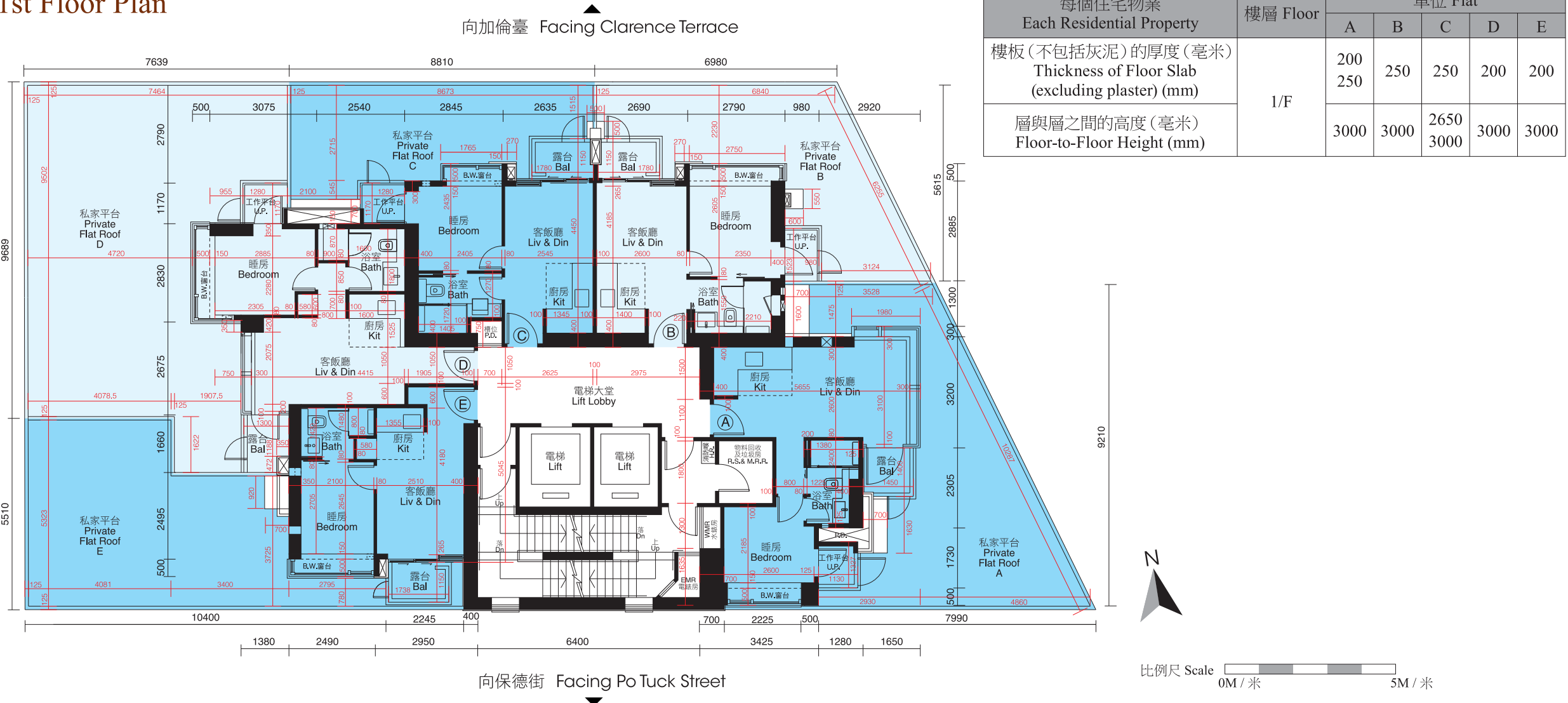
1樓平面圖 1st Floor Plan
