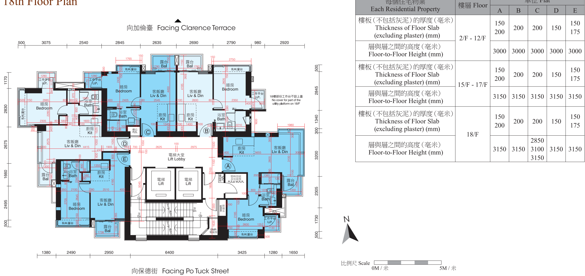
2樓至18樓平面圖 2nd to 18th Floor Plan
