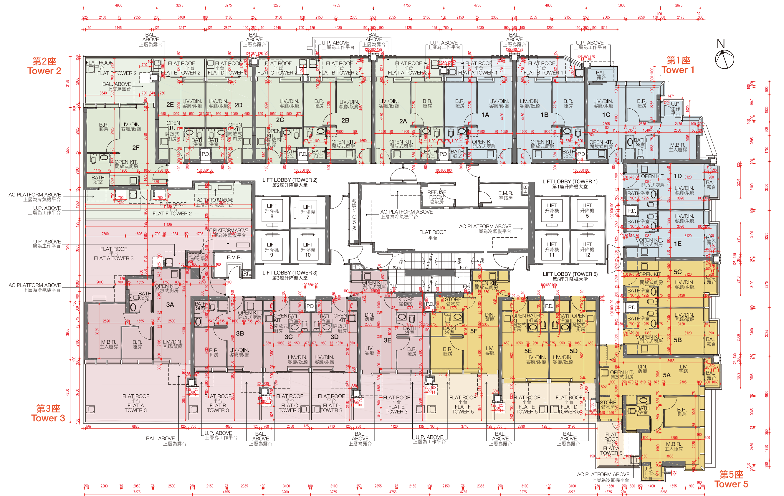
5樓平面圖 5th Floor Plan
