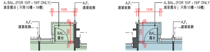
J單位露台部份平面圖 (10樓-12樓、15樓-23樓、25樓-33樓及35樓-36樓) BALCONY PART PLAN FOR FLAT J (10/F-12/F, 15/F-23/F, 25/F-33/F & 35/F-36/F)
