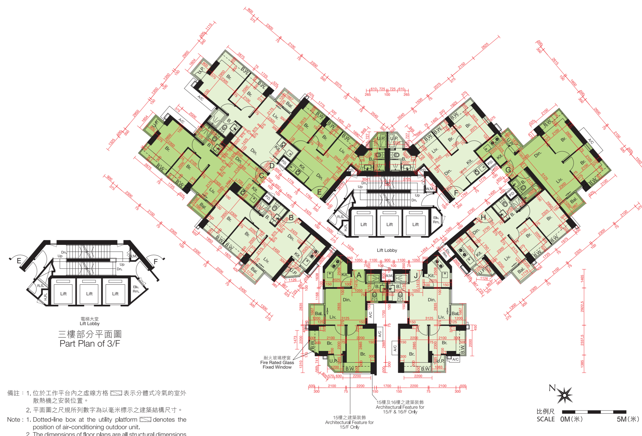
三樓至十六樓平面圖 3RD - 16TH FLOOR PLAN
