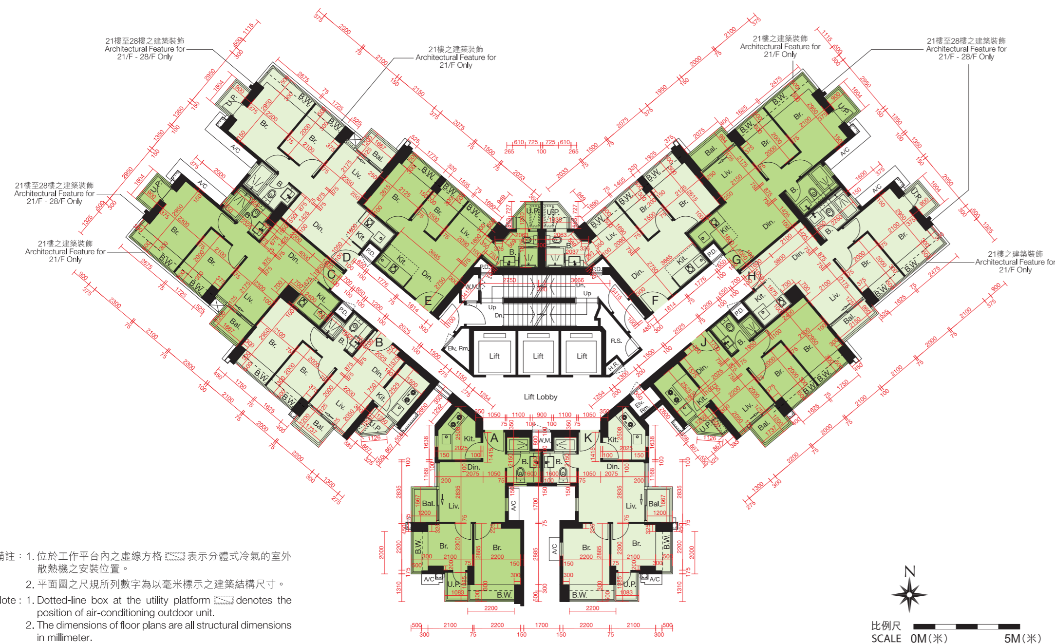
十七樓至二十八樓平面圖 17TH - 28TH FLOOR PLAN
