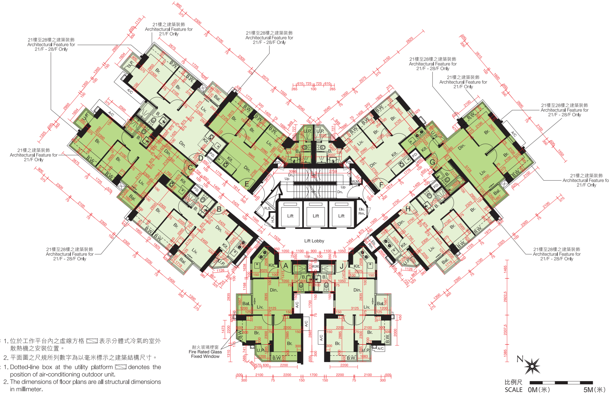
十七樓至二十八樓平面圖 17TH - 28TH FLOOR PLAN
