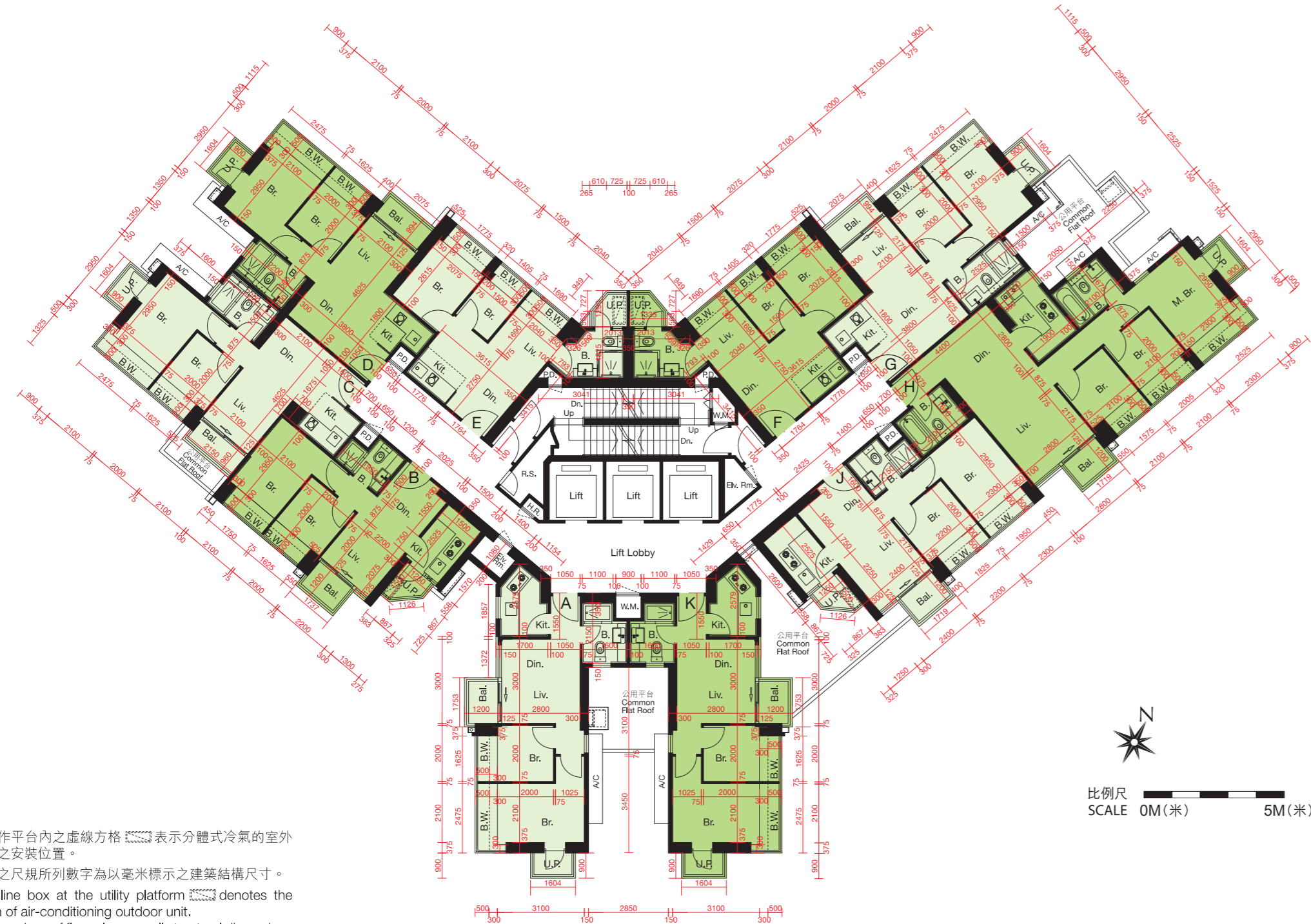
一樓平面圖 1ST FLOOR PLAN
