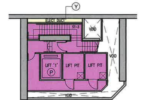
LIFT PIT PART PLAN
