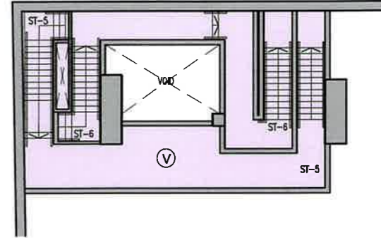
PART PLAN OF ST-5 AND ST-6
