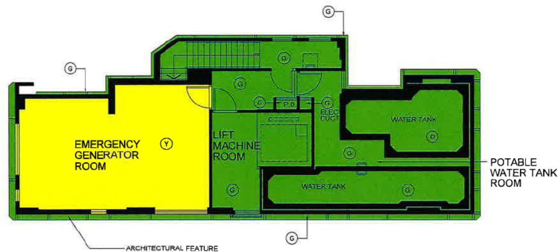
UPPER ROOF PLAN 2
