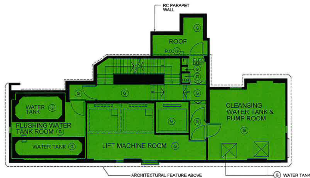
UPPER ROOF PLAN 1
