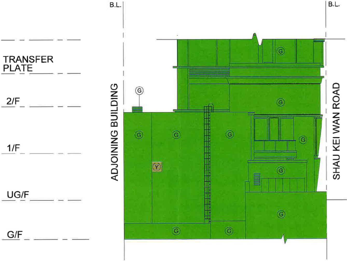
NORTH - WEST ELEVATION
